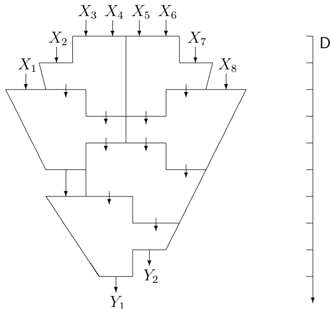
Figure 4.1: Multiple addition circuit of (3, 2) -compressors [258]
